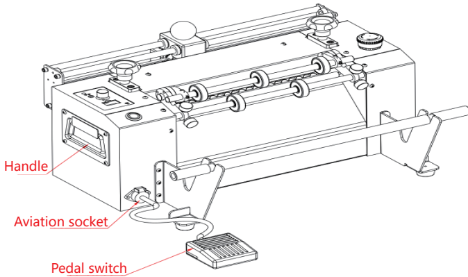
Figure 2 (Full view of the machine)
