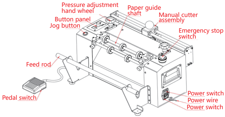
Figure 1 (Full view of the machine)
